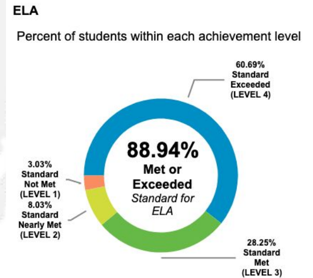
2018-19 ELA Scores
