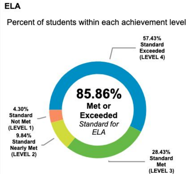
2016-17 ELA Scores
