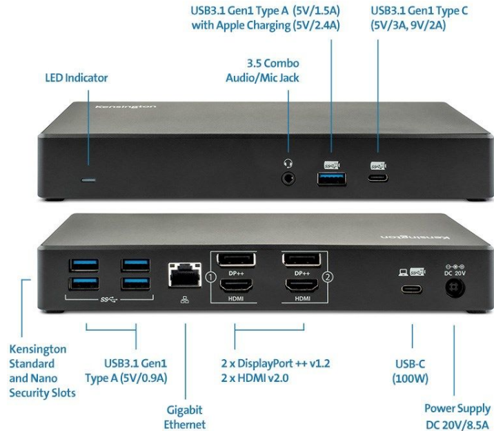
Kensington SD4780P Docking Station
